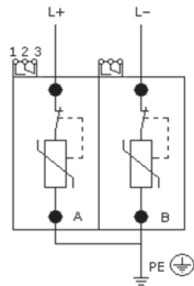
2 Pole - Photovoltaic
