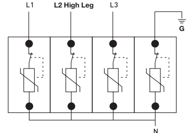
3 Phase Delta High-Leg 4 Pole - 5 Wire
