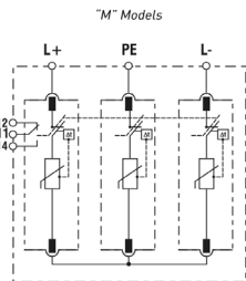
3 Poles
