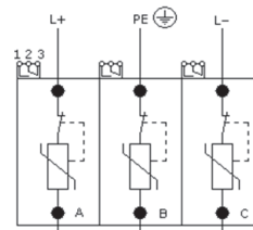
3 Pole - Photovoltaic
