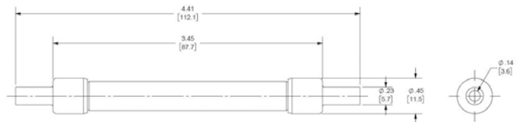
CC terminal: Recommended crimping tool: T & B Sta-Kon ERG4002 #10 -12 AWG (6-4 mm 2 )
