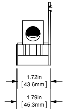
BACK VIEW ADDER (MPDB67010) SHOWN
